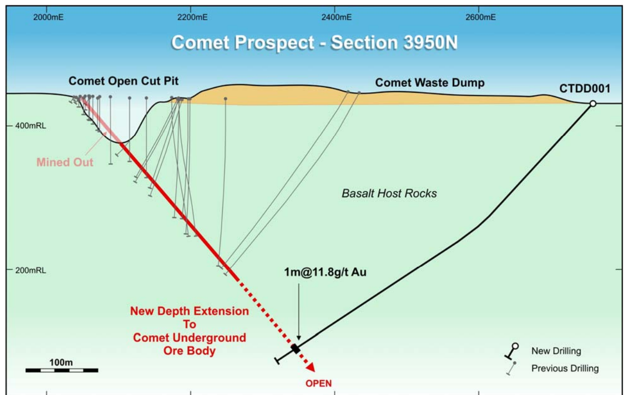
Figure 1. Geological cross section showing the location of the gold mineralised structure down-dip from previous resource drilling.
